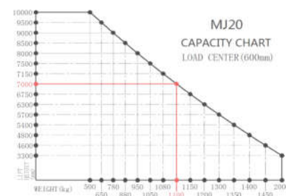
Capacity Chart-MJ20
