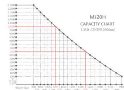
Capacity Chart-MJ20H
